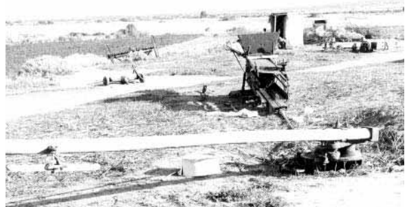
Baling system powered by horses that turn the long shaft, Ebenhaeser, Western Cape
