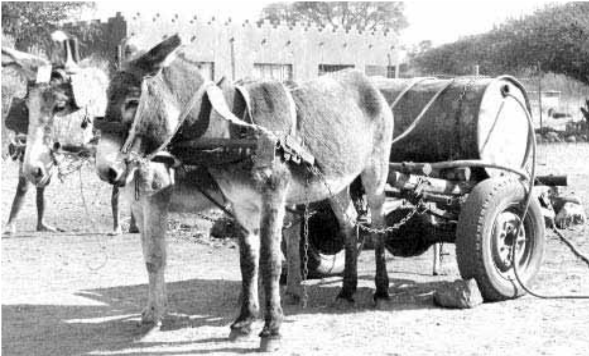
This locally-made donkey-drawn cart has been specially designed for water transportation in North-West Province (Bophuthatswana)
